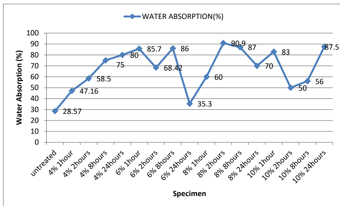
Fig. 1. Water absorption of Oil Palm Broom Fibre.
