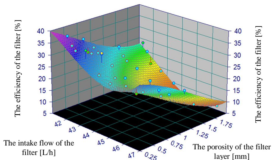
Fig. 3. Tridimensional representations of the filtering process efficiency for the filter with perlite [12].
